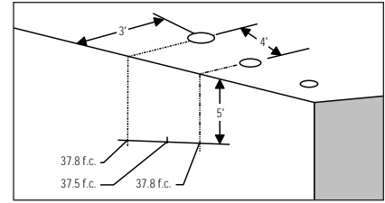
Lighting Data - Example C6T6WCLW illumination on the wall 5' down from the ceiling is 37.8 f.c. beneath and 37.5 f.c. between fixtures.
